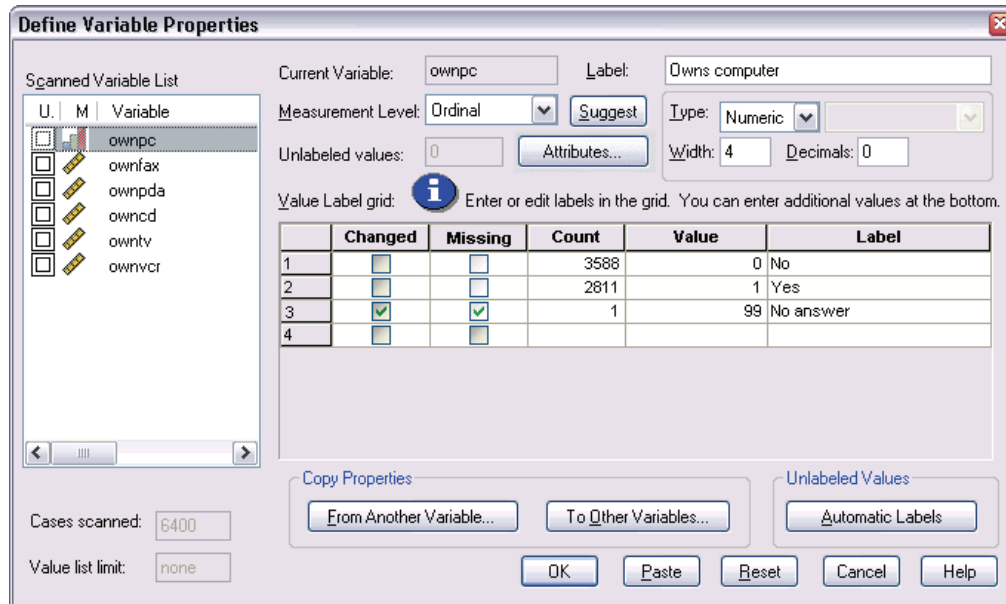
Figure 3-23 New variable properties defined for ownpc
