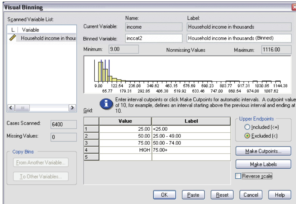
Figure 9-5 Automatically generated value labels
