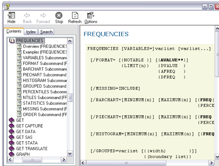
Figure 8-4 FREQUENCIES syntax help
