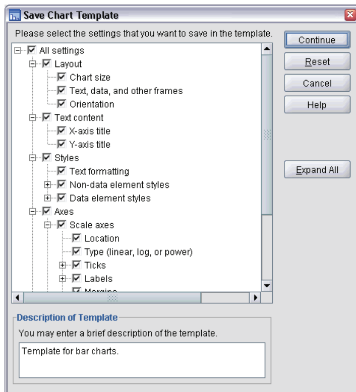
Figure 6-15 Save Chart Template dialog box
