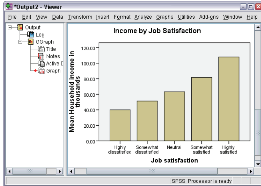
Figure 6-6 Bar chart
