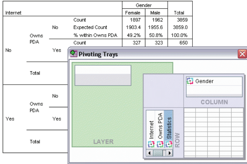
Figure 7-4 Pivoting trays
