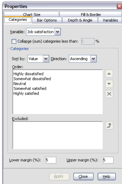
Figure 6-8 Properties window
