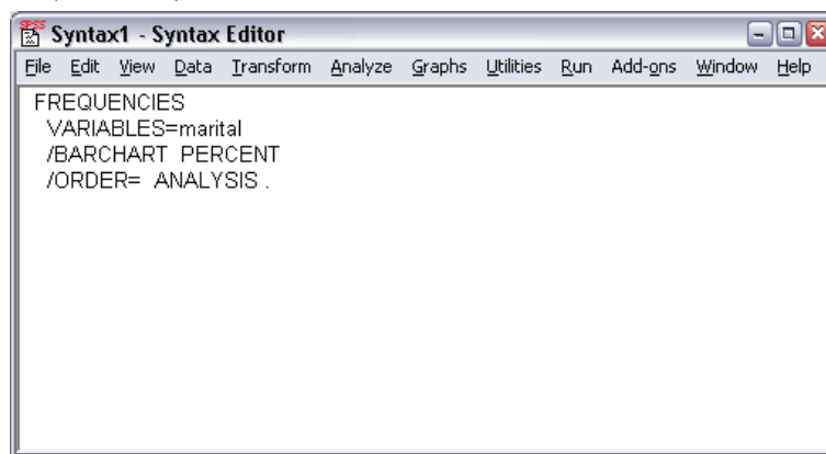
Figure 8-2 Frequencies syntax
