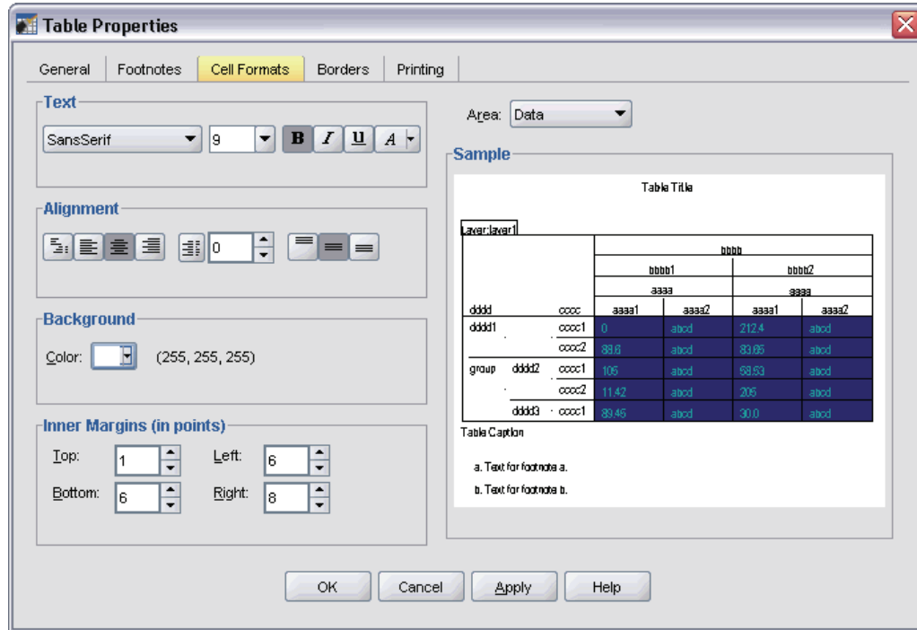
Figure 7-15 Changing table cell formats
