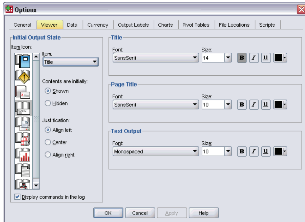
Figure 7-18 Viewer options
