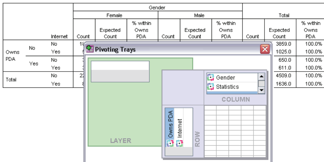
Figure 7-6 Swap rows
